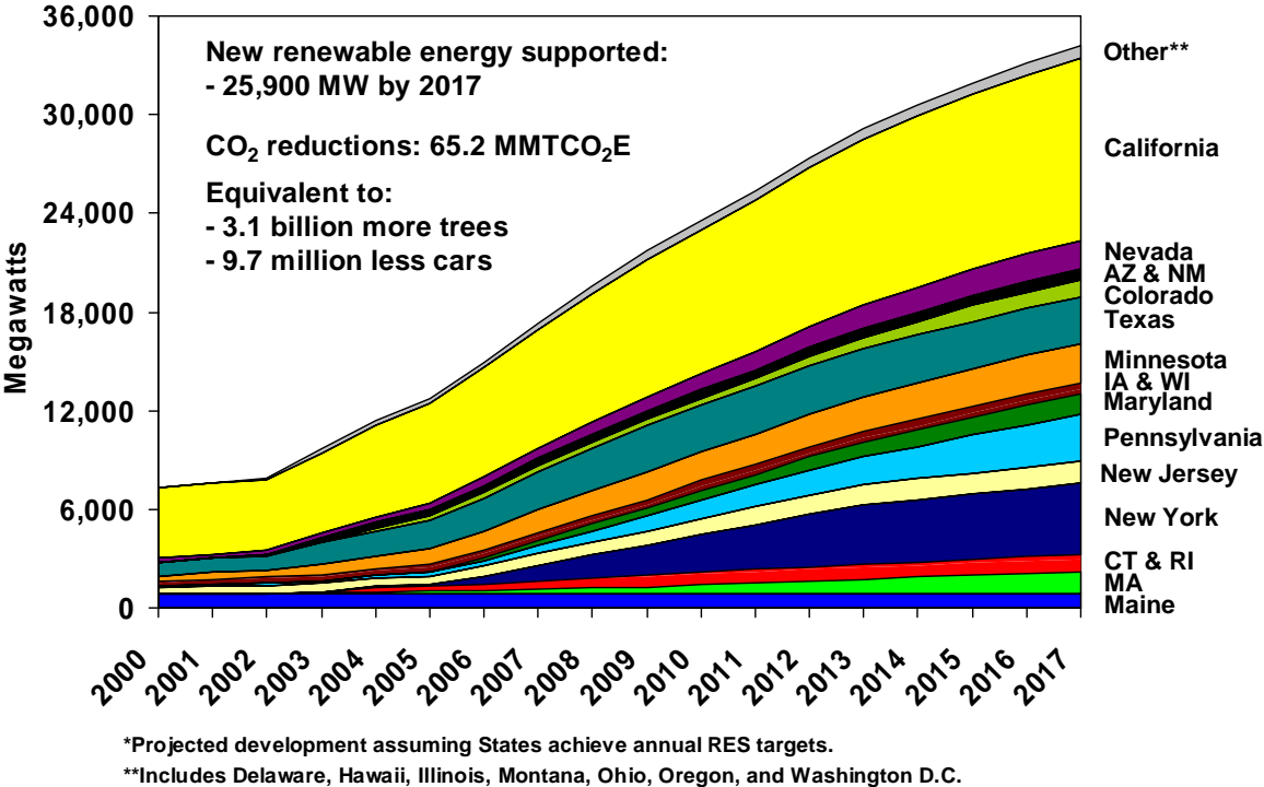
Fig. 14: Prediction of new Renewables from State Standards and Renewable Energy Funds Figure © Union of Concerned Scientists [Uni 2005b]
